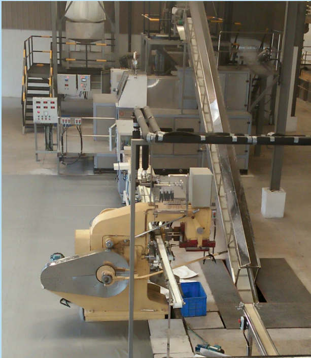
Automatic Soaps Stamping Machine
